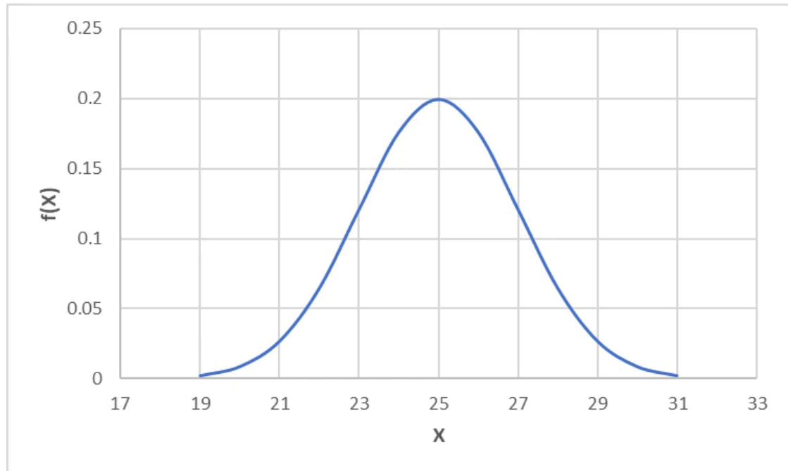
Figure 3: Normal Distribution Curve
