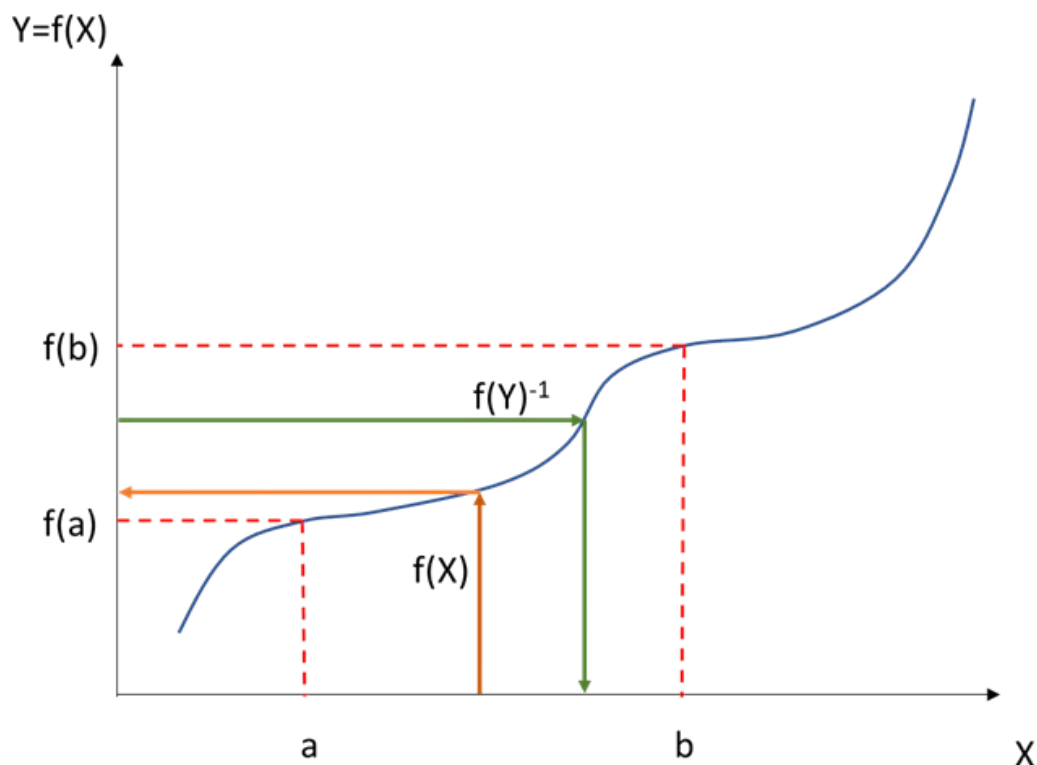
Figure 3: A Strictly Increasing Function Example
